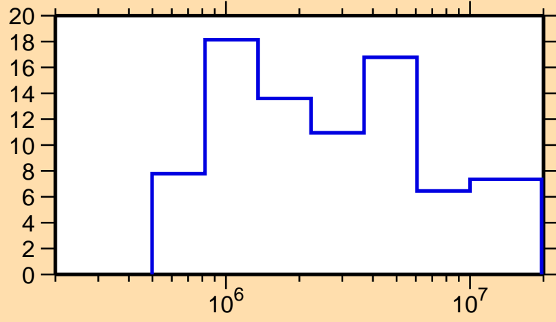
\Delta\sigma/\sigma vs. E for ^{186}\text{Re}(n, el.)
