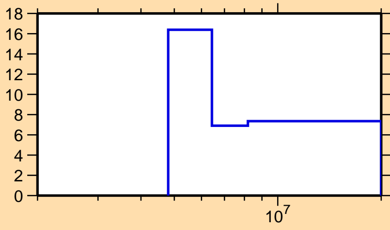
\Delta\sigma/\sigma vs. E for ^{186}\text{Re}(n,\text{el.})
