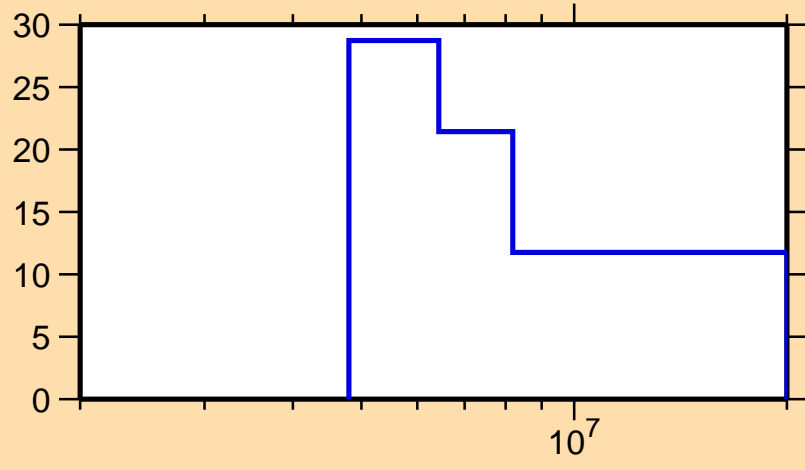
\Delta\sigma/\sigma vs. E for ^{186}\text{Re}(n,2n)
