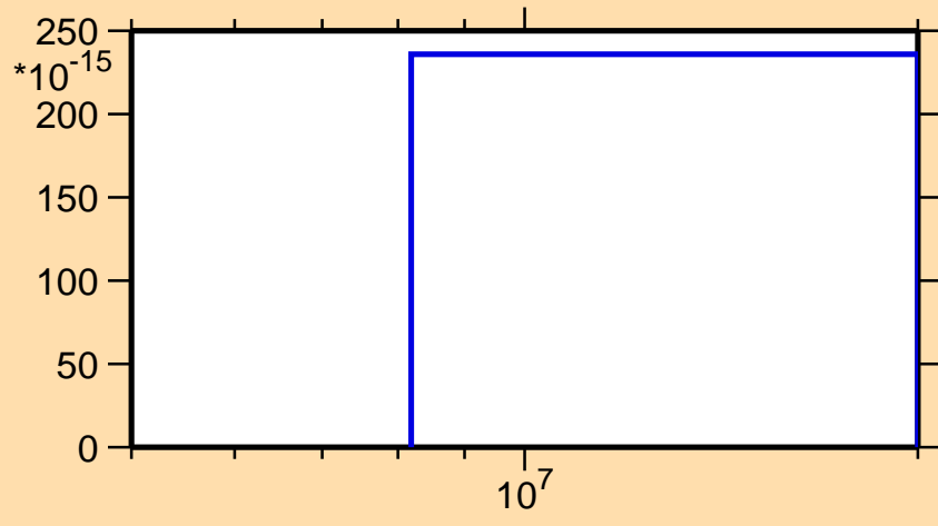
\sigma vs. E for ^{186}\text{Re}(n,p\alpha)
