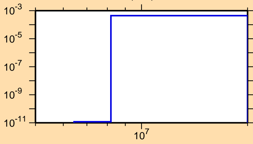
\sigma vs. E for ^{186}\text{Re}(n,d)
