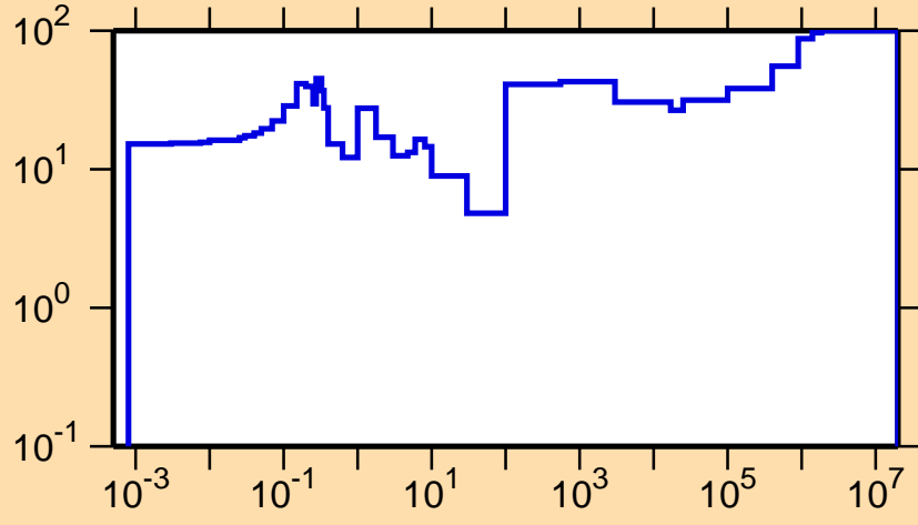
\Delta\sigma/\sigma vs. E for ^{186}\text{Re}(n,\gamma)
