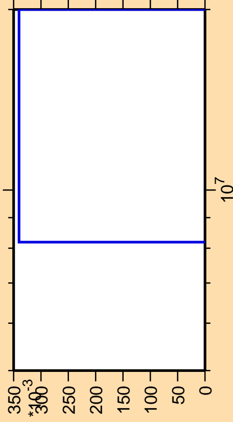
\Delta\sigma/\sigma vs. E for ^{186}\text{Re}(n,p\alpha)
