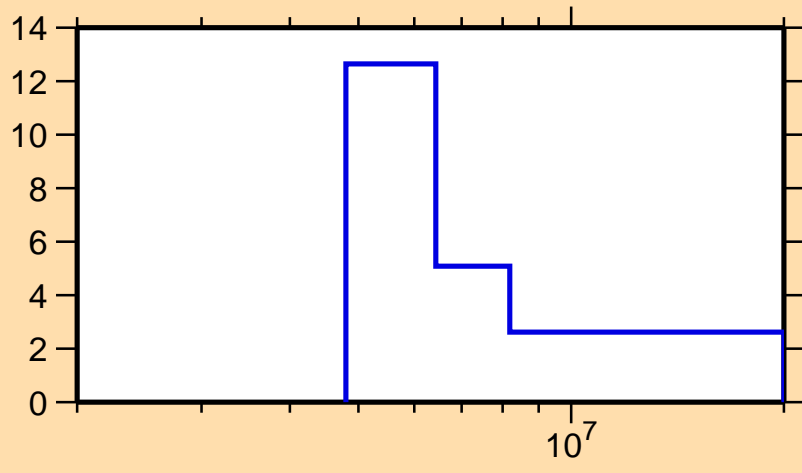
\Delta\sigma/\sigma vs. E for ^{186}\text{Re}(n,\text{tot.})
