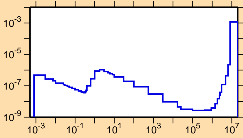
\sigma vs. E for ^{186}\text{Re}(n,\alpha)
