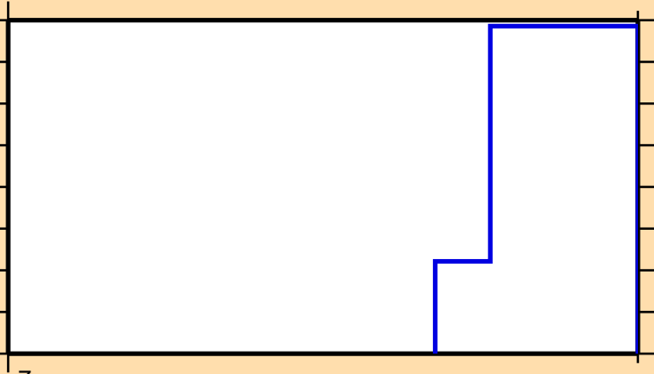
\sigma vs. E for ^{186}\text{Re}(n,p\alpha)
