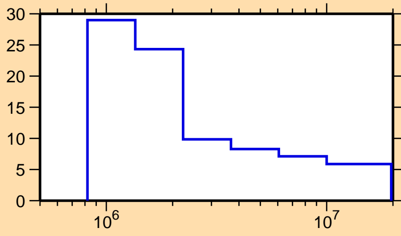
\Delta\sigma/\sigma vs. E for ^{186}\text{Re}(n,\text{nonel.})
