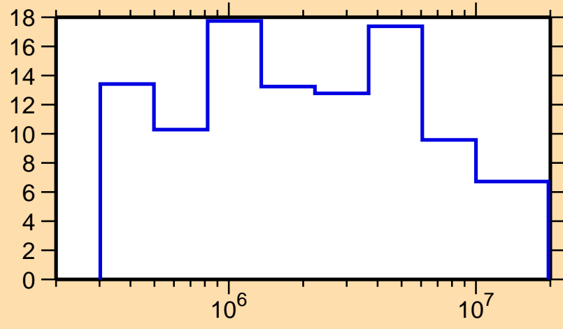
\Delta\sigma/\sigma vs. E for ^{186}\text{Re}(n, el.)
