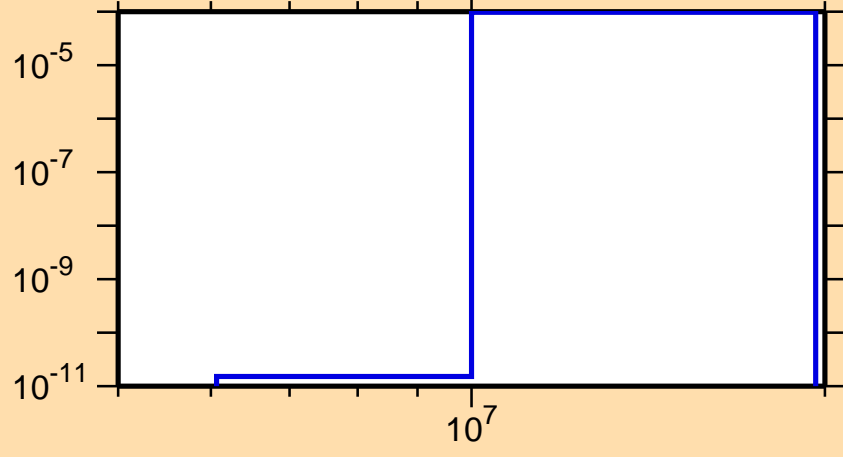
\sigma vs. E for ^{186}\text{Re}(n,t)
