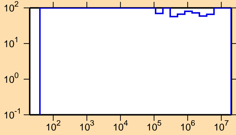
\Delta\sigma/\sigma vs. E for ^{186}\text{Re}(n,n_1)
