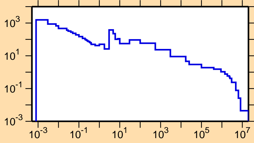
\sigma vs. E for ^{186}\text{Re}(n,\gamma)
