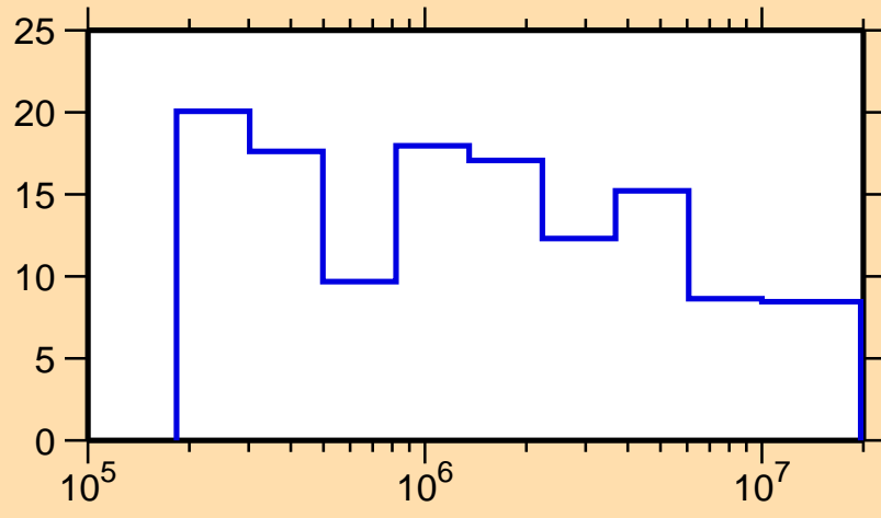
\Delta\sigma/\sigma vs. E for ^{188}\text{Re}(n, el.)
