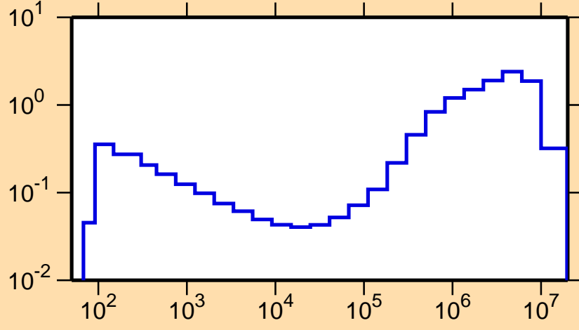
\sigma vs. E for ^{188}\text{Re}(n,\text{inel.})
