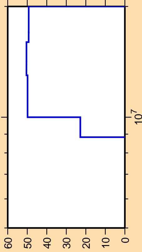
\Delta\sigma/\sigma vs. E for ^{189}\text{Re}(n,np)
