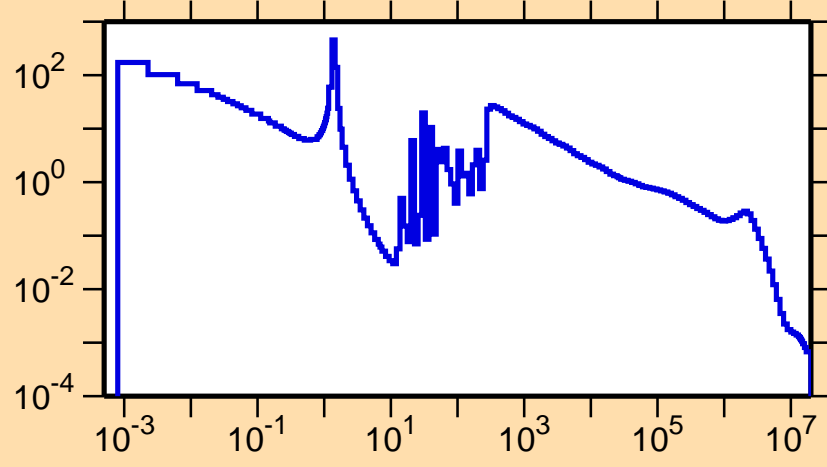
\sigma vs. E for ^{189}\text{Re}(n,\gamma)
