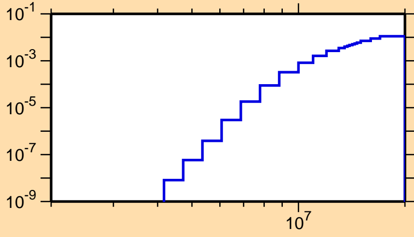
\sigma vs. E for ^{190}\text{Re}(n,p)
