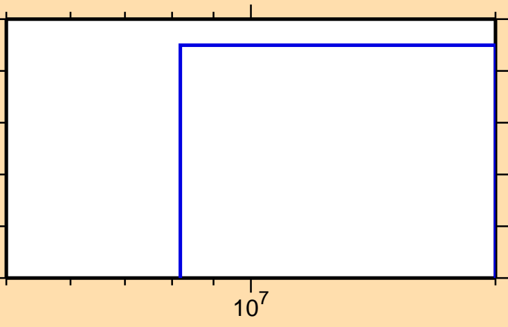
\sigma vs. E for ^{190}\text{Re}(n,3n)
