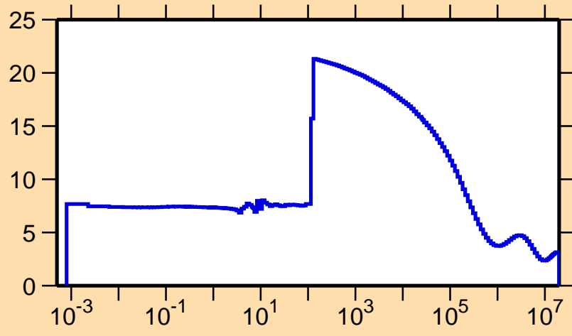
\sigma vs. E for ^{190}\text{Re}(n,\text{el.})
