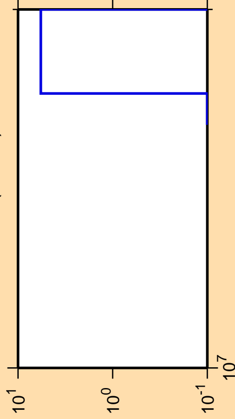
\Delta\sigma/\sigma vs. E for ^{190}\text{Re}(n,\text{He3})
