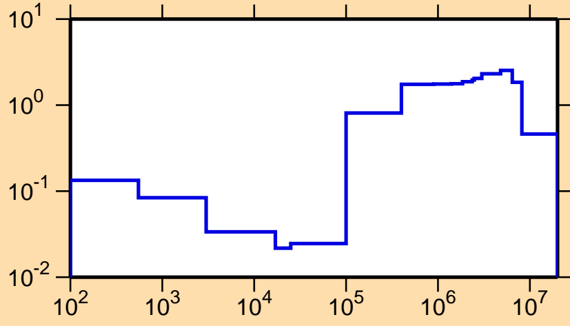
\sigma vs. E for ^{190}\text{Re}(n,\text{inel.})
