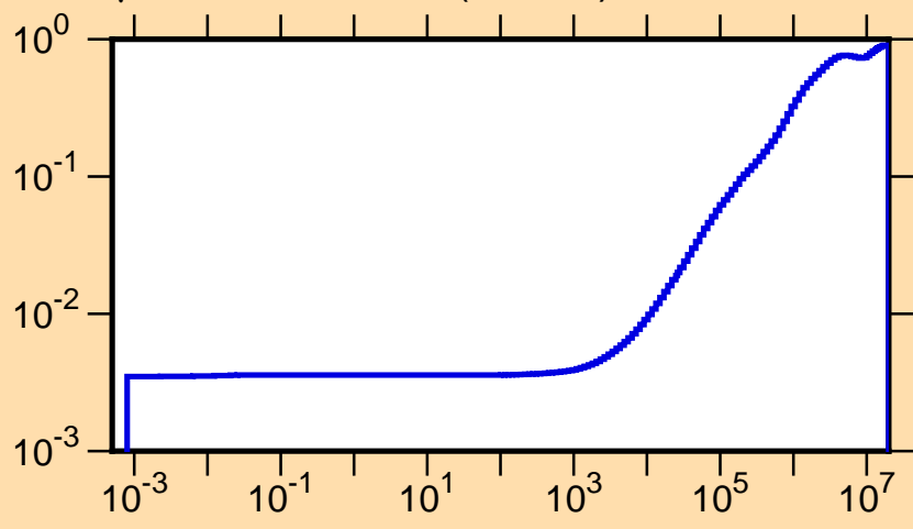
\mu vs. E for ^{193}\text{Re}(\text{mt251})
