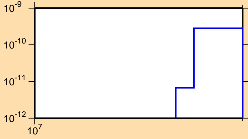
\sigma vs. E for ^{193}\text{Re}(n,2n\alpha)
