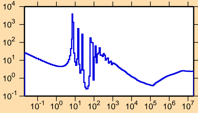
\sigma vs. E for ^{193}\text{Re}(n,\text{nonel.})
