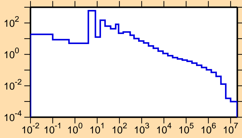
\sigma vs. E for ^{193}\text{Re}(n,\gamma)
