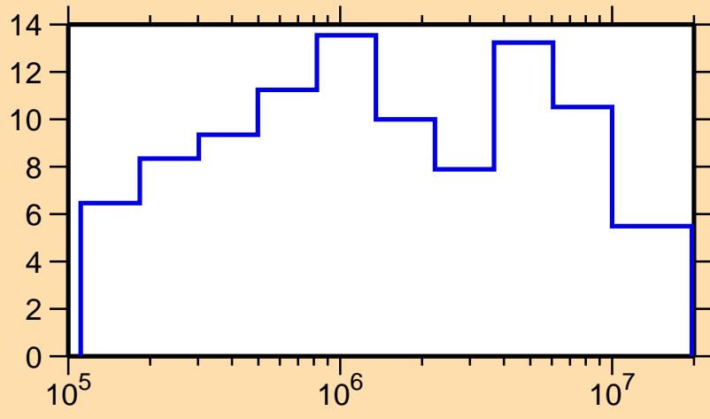
\Delta\sigma/\sigma vs. E for ^{193}\text{Re}(n, el.)
