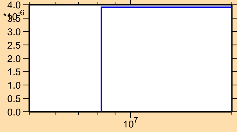
\sigma vs. E for ^{193}\text{Re}(n,t)
