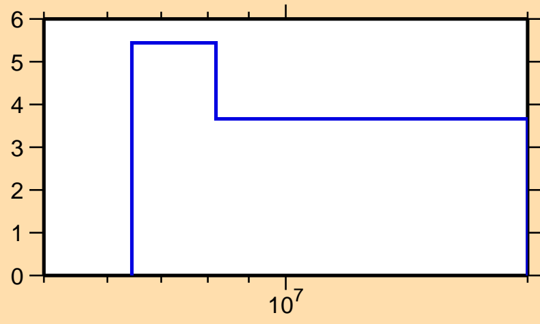
\Delta\sigma/\sigma vs. E for ^{193}\text{Re}(n,\text{tot.})
