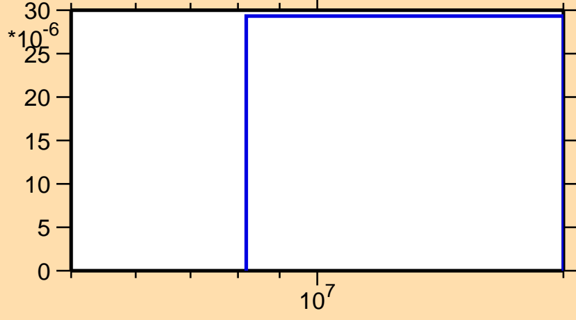
\sigma vs. E for ^{193}\text{Re}(n,d)
