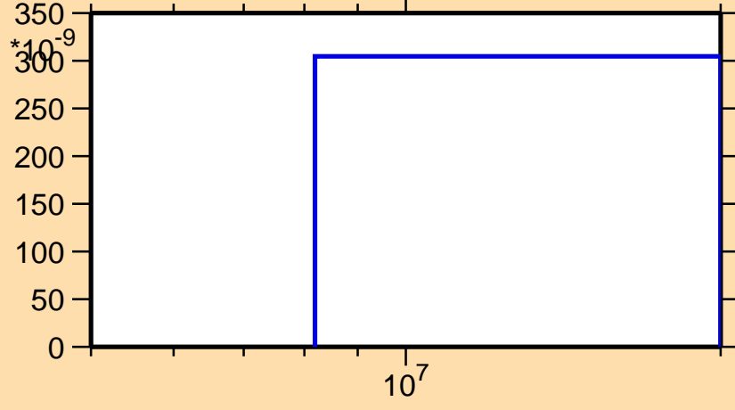
\sigma vs. E for ^{193}\text{Re}(n,n\alpha)
