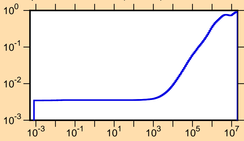
\mu vs. E for ^{194}\text{Re}(\text{mt251})
