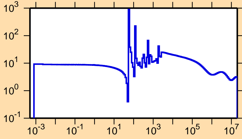
\sigma vs. E for ^{194}\text{Re}(n,\text{el.})
