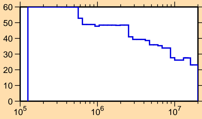
\Delta\sigma/\sigma vs. E for ^{194}\text{Re}(n,n\text{onel.})
