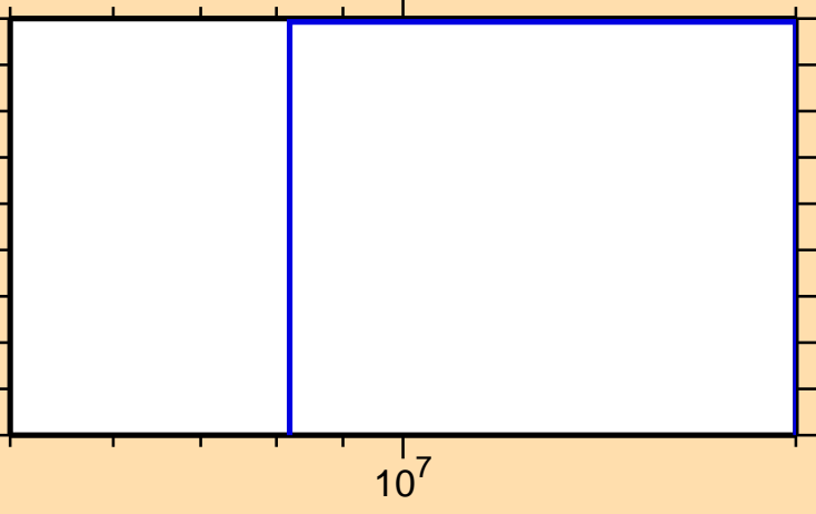
\sigma vs. E for ^{194}\text{Re}(\text{mt } 42)
