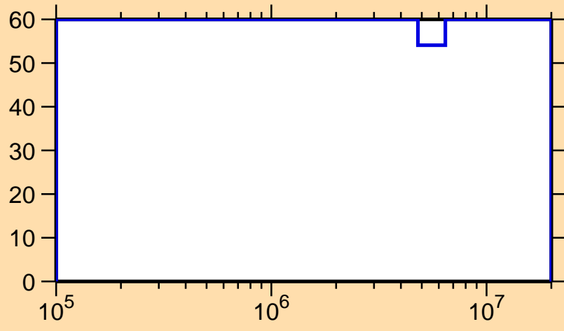
\Delta\sigma/\sigma vs. E for ^{194}\text{Re}(n,n_1)
