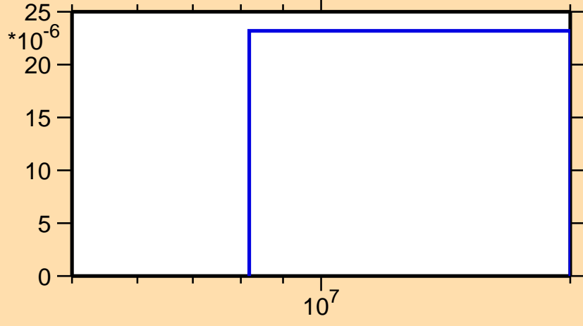
\sigma vs. E for ^{194}\text{Re}(n,np)
