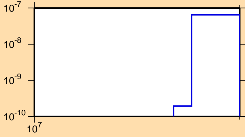
\sigma vs. E for ^{195}\text{Re}(n,\text{nd})
