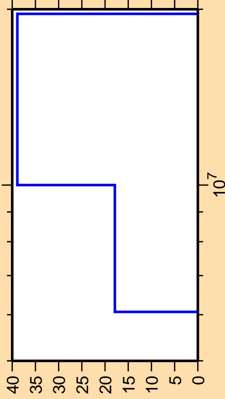
\Delta\sigma/\sigma vs. E for ^{195}\text{Re}(n,2n)
