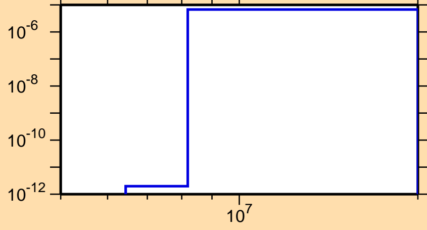
\sigma vs. E for ^{195}\text{Re}(n,\alpha)
