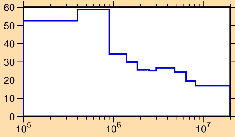
\Delta\sigma/\sigma vs. E for ^{195}\text{Re}(n,n\text{nonel.})
