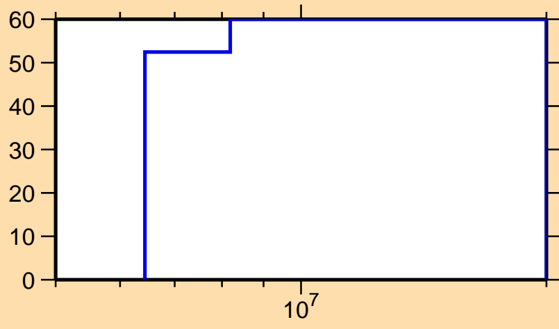
\Delta\sigma/\sigma vs. E for ^{195}\text{Re}(n,ncont.)
