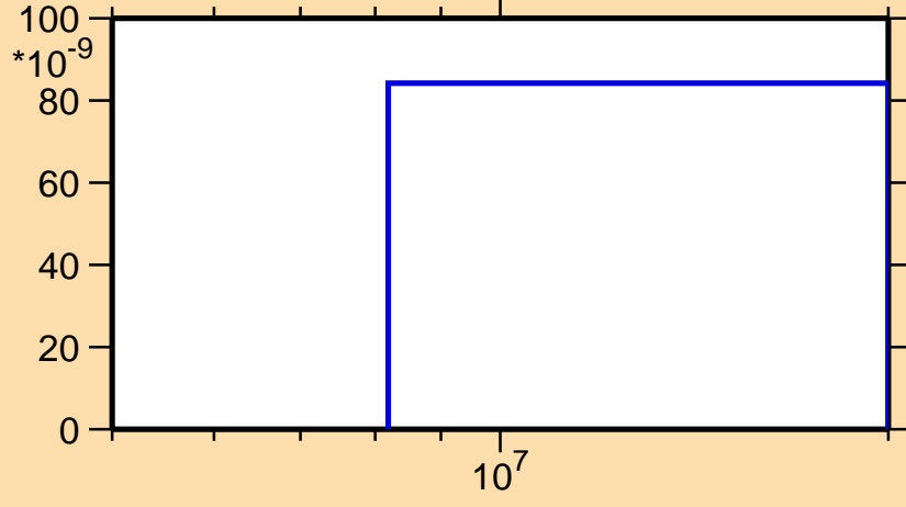
\sigma vs. E for ^{195}\text{Re}(n,n\alpha)
