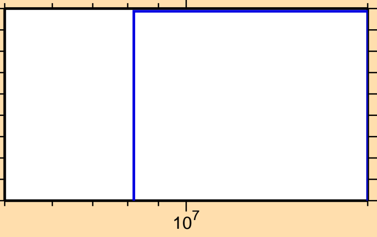
\sigma vs. E for ^{195}\text{Re}(\text{mt } 42)
