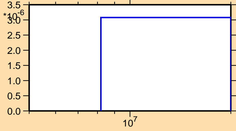
\sigma vs. E for ^{195}\text{Re}(n,t)
