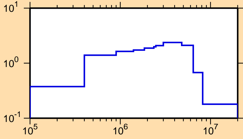
\sigma vs. E for ^{196}\text{Re}(n,\text{inel.})
