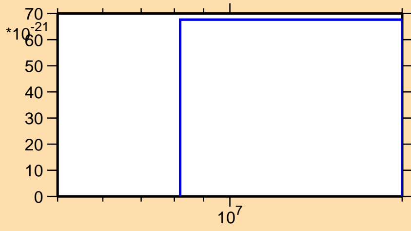
\sigma vs. E for ^{196}\text{Re}(\text{mt } 42)
