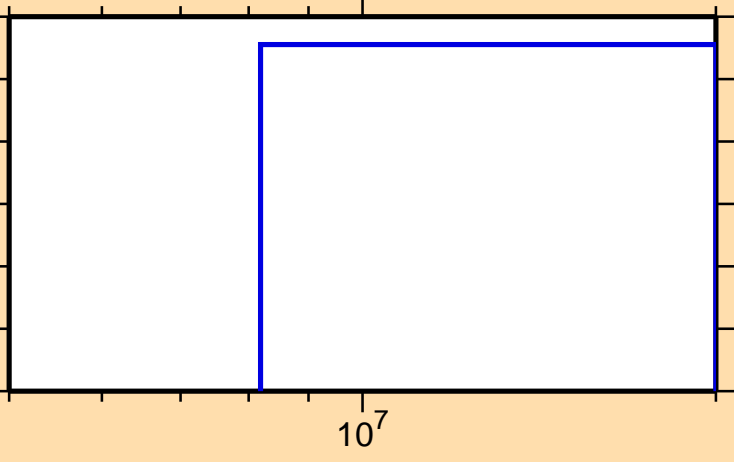
\sigma vs. E for ^{196}\text{Re}(n,\text{nd})
