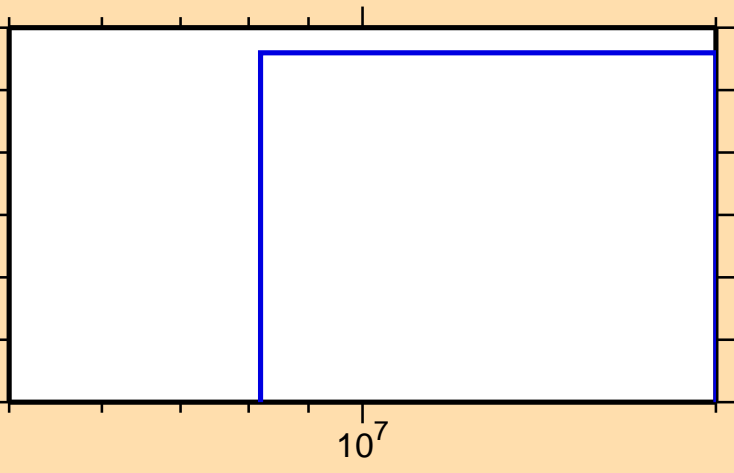
\sigma vs. E for ^{196}\text{Re}(n,2np)
