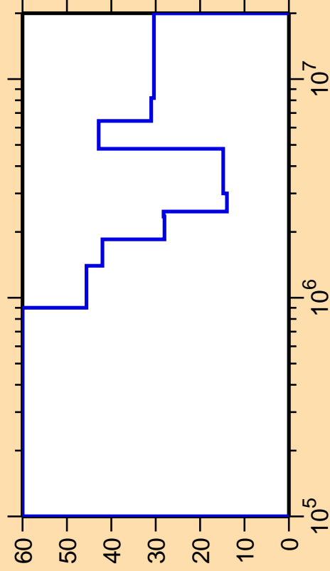
\Delta\sigma/\sigma vs. E for ^{196}\text{Re}(n,\text{inel.})
