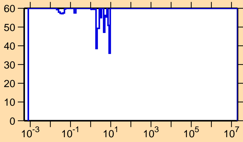
\Delta\sigma/\sigma vs. E for ^{255}\gamma
