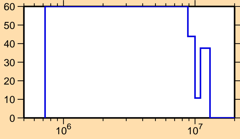
\Delta\sigma/\sigma vs. E for ^{255}_{1}\text{Pu}
