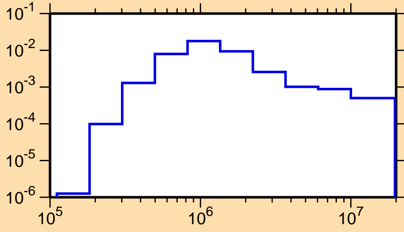
\sigma vs. E for ^{257}_{3}
