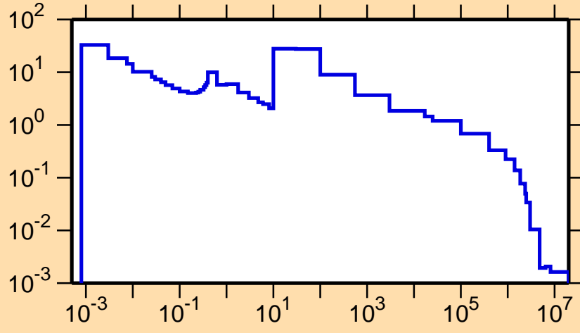
\sigma vs. E for ^{259}\text{Pu} \gamma
