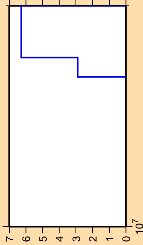
\Delta\sigma/\sigma vs. E for ^{264}\alpha )
