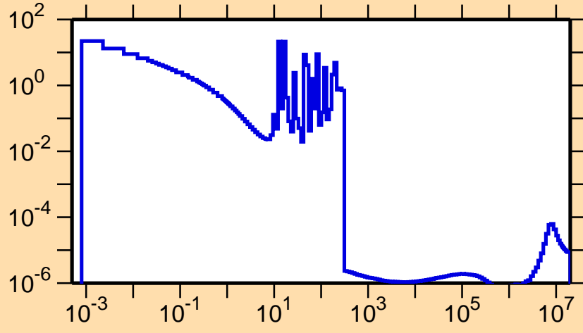
\sigma vs. E for ^{268}\gamma
