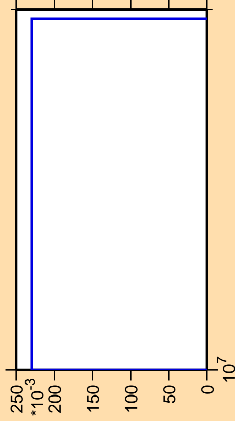
\Delta\sigma/\sigma vs. E for ^{280}
