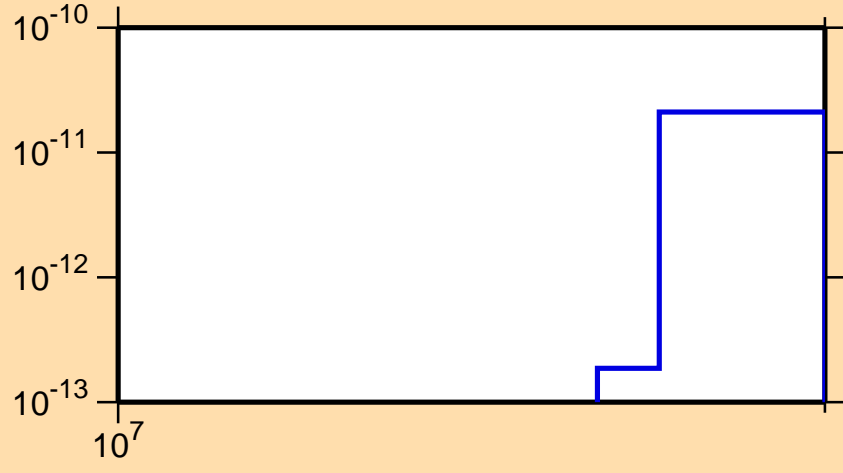
\sigma vs. E for ^{283}\text{He3}
