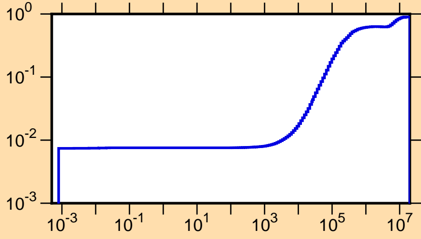
\mu vs. E for ^{91}\text{Rh}(\text{mt251})
