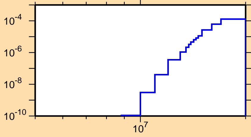
\sigma vs. E for ^{91}\text{Rh}(n,\alpha)
