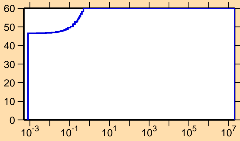
\Delta\sigma/\sigma vs. E for ^{91}\text{Rh}(n,\gamma)
