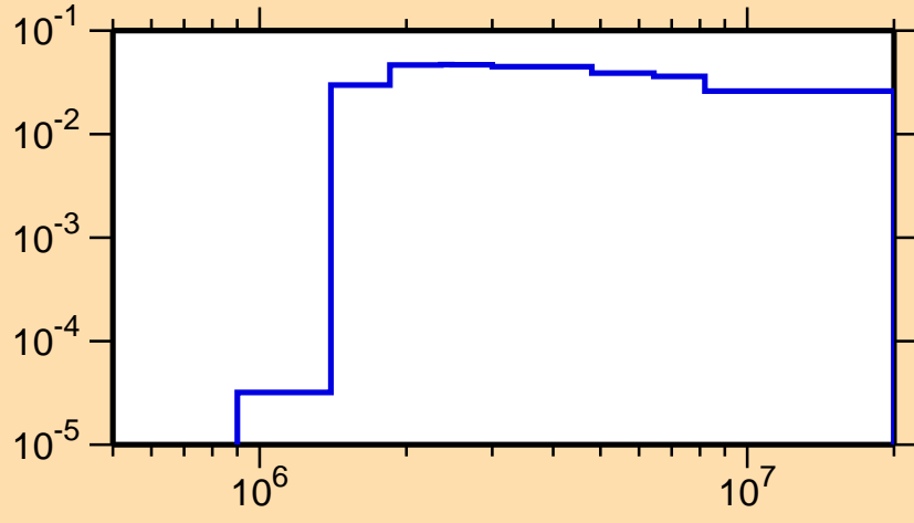
\sigma vs. E for ^{91}\text{Rh}(n,n_4)
