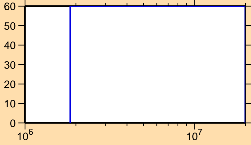
\Delta\sigma/\sigma vs. E for ^{92}\text{Rh}(n,n\text{cont.})
