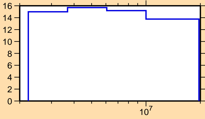
\Delta\sigma/\sigma vs. E for ^{94}\text{Rh}(n,n\text{nonel.})
