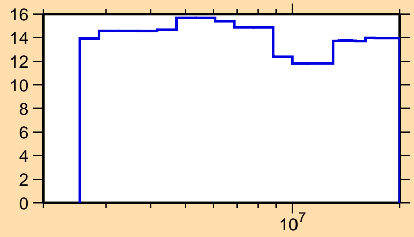
\Delta\sigma/\sigma vs. E for ^{94}\text{Rh}(n,n\text{onel.})
