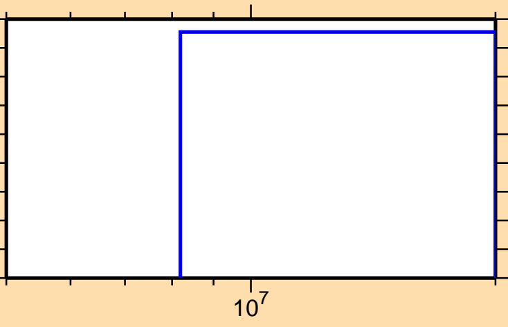
\sigma vs. E for ^{94}\text{Rh}(n,2n)
