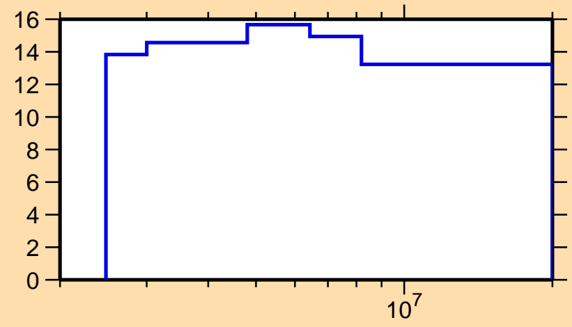
\Delta\sigma/\sigma vs. E for ^{94}\text{Rh}(n,n\text{nonel.})
