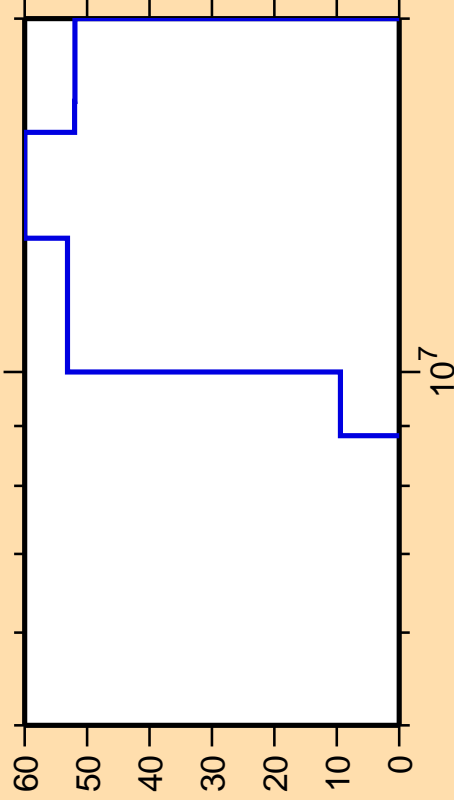
\Delta\sigma/\sigma vs. E for ^{95}\text{Rh}(n,\alpha)
