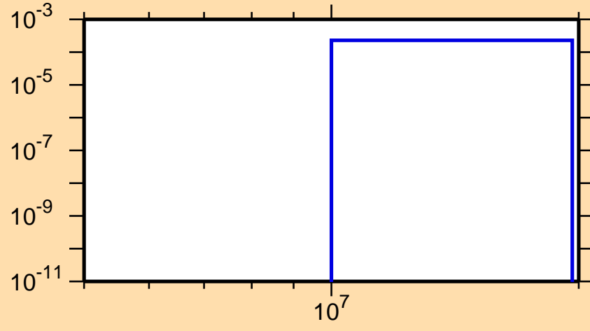
\sigma vs. E for ^{95}\text{Rh}(n,n\alpha)
