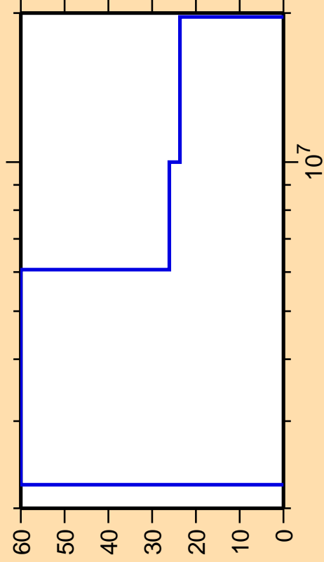
\Delta\sigma/\sigma vs. E for ^{95}\text{Rh}(n,n\text{cont.})
