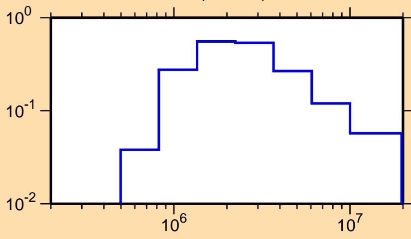
\sigma vs. E for ^{95}\text{Rh}(n,\text{inel.})
