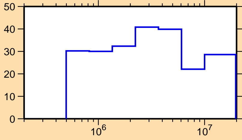
\Delta\sigma/\sigma vs. E for ^{95}\text{Rh}(n,n_1)
