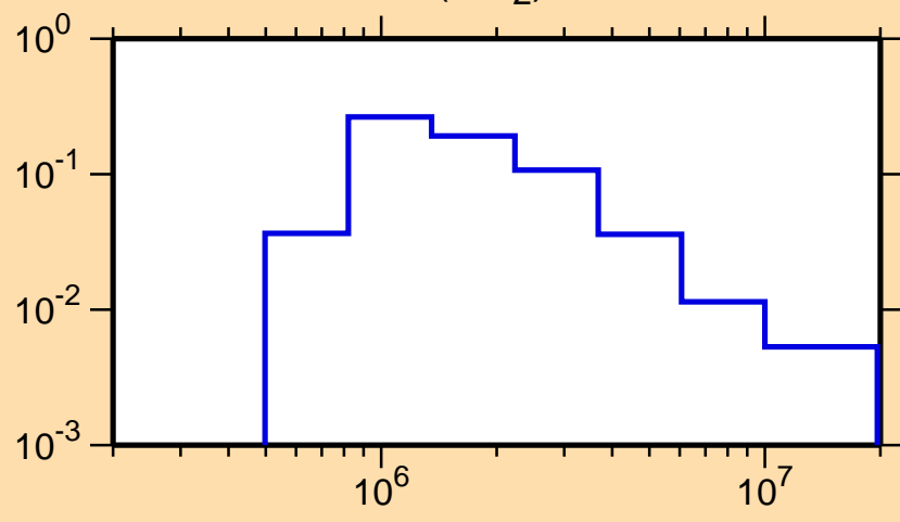
\sigma vs. E for ^{95}\text{Rh}(n,n_2)
