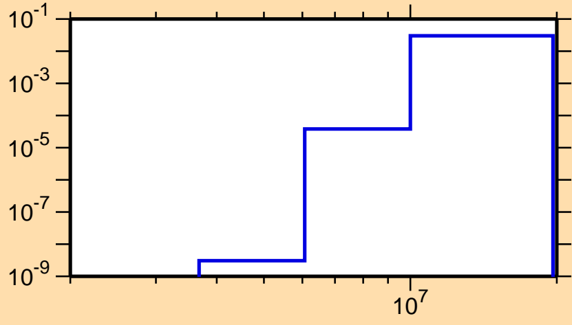
\sigma vs. E for ^{95}\text{Rh}(n,p\alpha)
