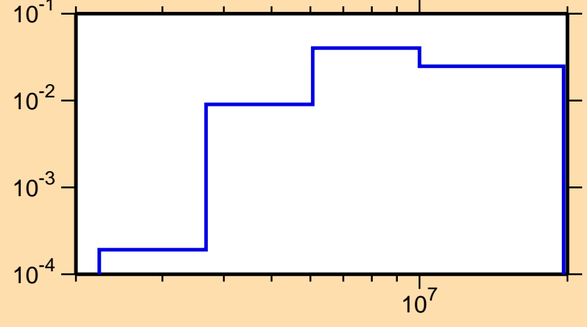
\sigma vs. E for ^{95}\text{Rh}(n,n\text{cont.})
