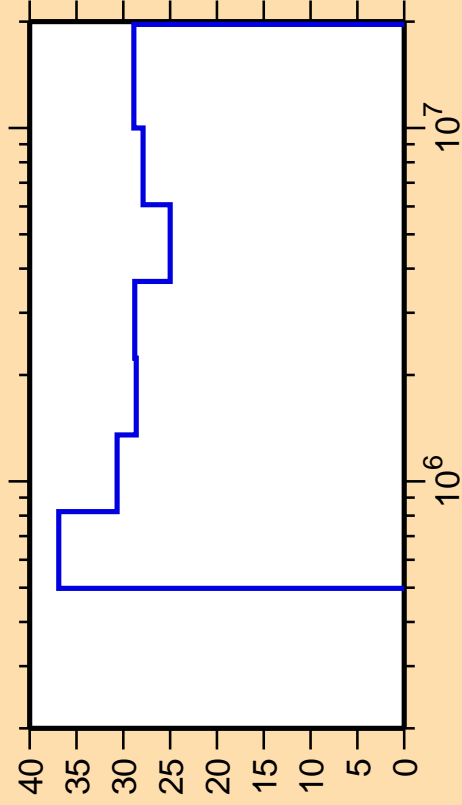
\Delta\sigma/\sigma vs. E for ^{95}\text{Rh}(n,n_2)
