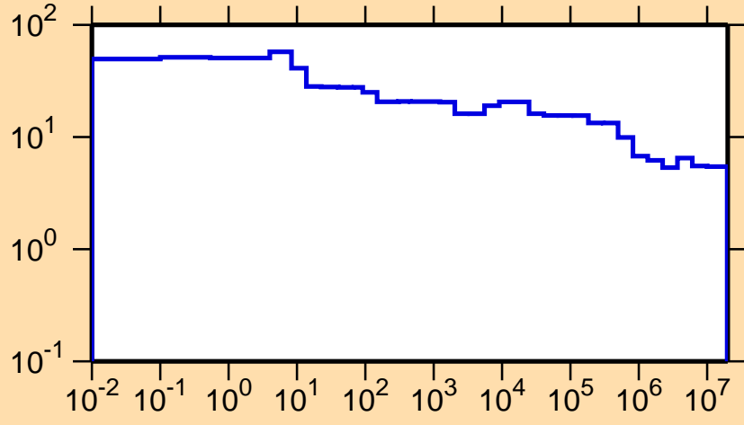
\Delta\sigma/\sigma vs. E for ^{95}\text{Rh}(n,\text{nonel.})
