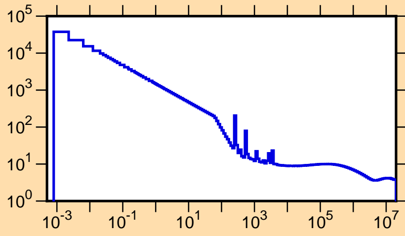
\sigma vs. E for ^{95}\text{Rh}(n,\text{tot.})
