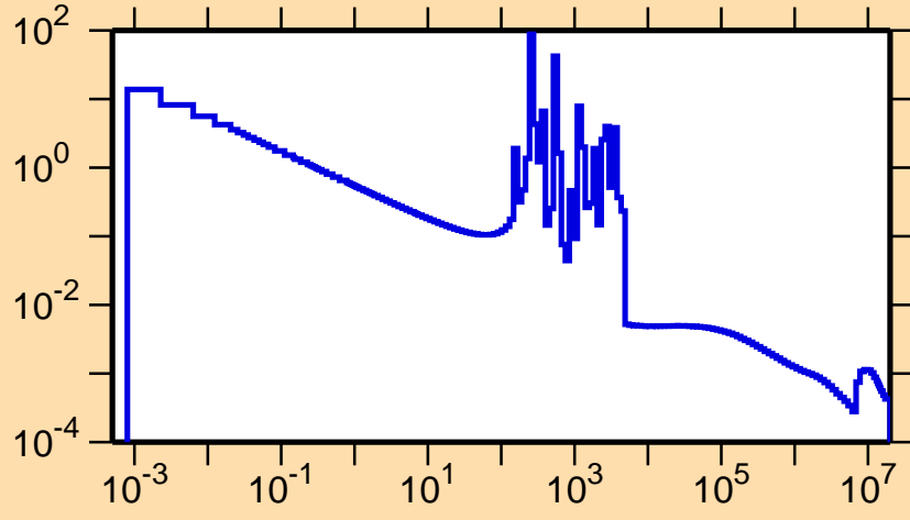
\sigma vs. E for ^{95}\text{Rh}(n,\gamma)
