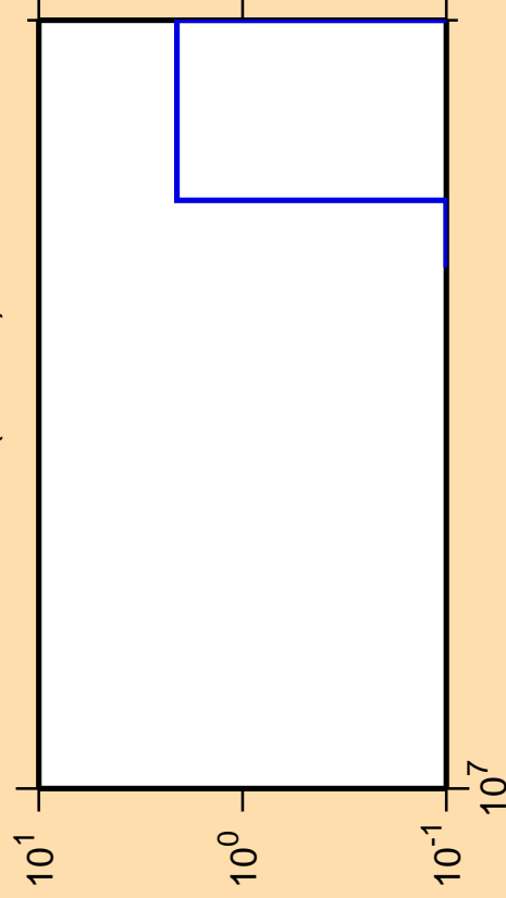
\Delta\sigma/\sigma vs. E for ^{95}\text{Rh} (mt 34)
