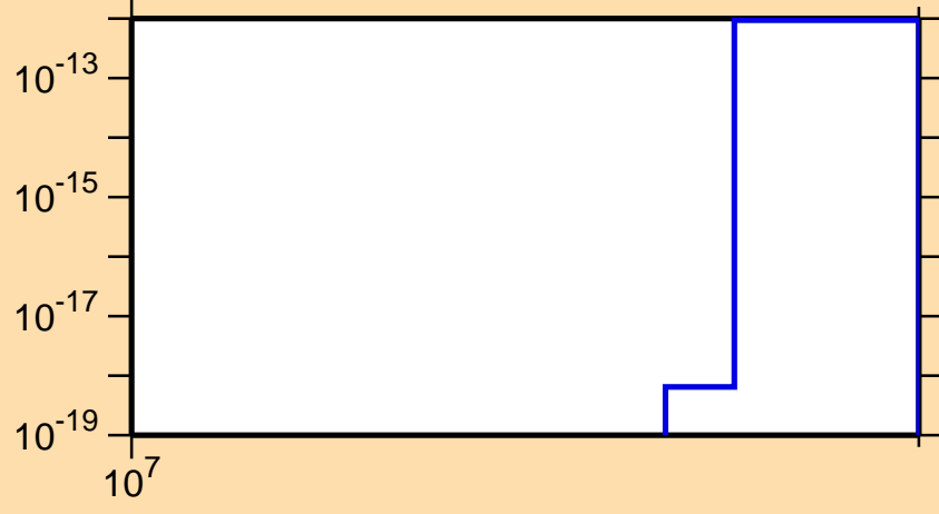
\sigma vs. E for ^{95}\text{Rh} (mt 34)
