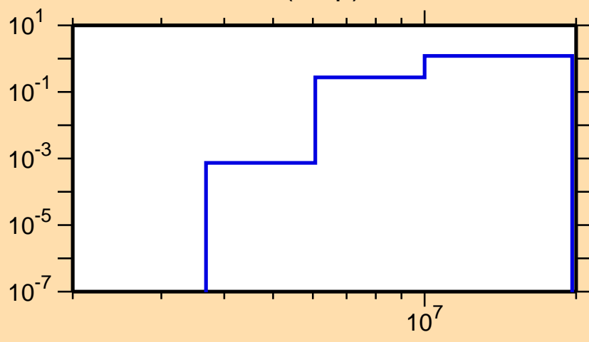
\sigma vs. E for ^{95}\text{Rh}(n,np)
