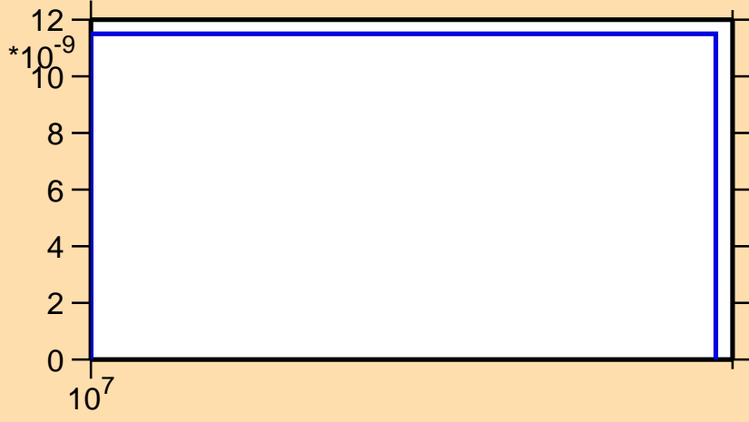
\sigma vs. E for ^{95}\text{Rh}(\text{mt } 45)
