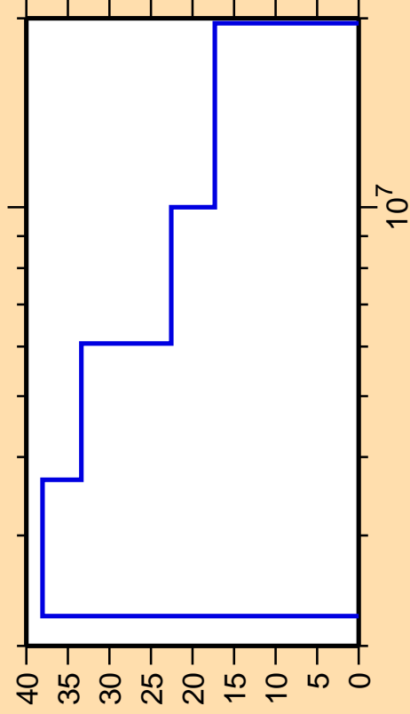
\Delta\sigma/\sigma vs. E for ^{95}\text{Rh}(n,np)
