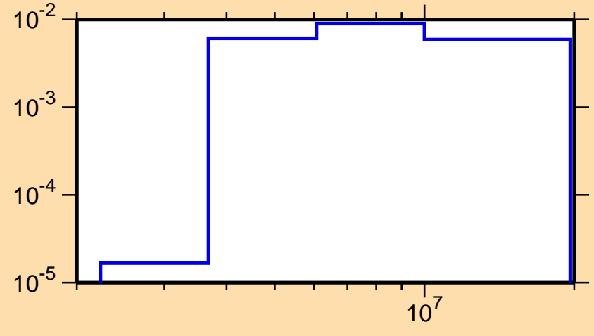
\sigma vs. E for ^{95}\text{Rh}(n,n\text{cont.})
