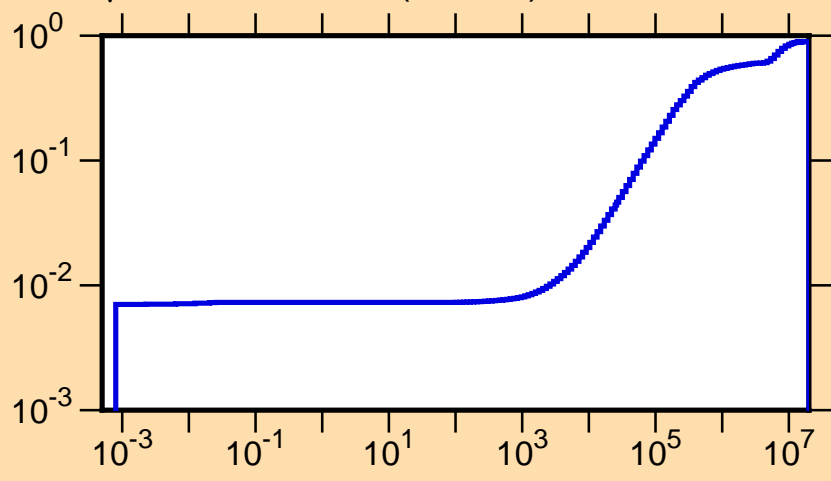
\mu vs. E for ^{96}\text{Rh}(\text{mt251})
