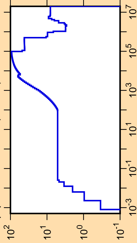
\Delta\mu/\mu vs. E for ^{96}\text{Rh}(\text{mt251})
