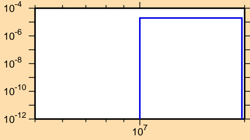
\sigma vs. E for ^{96}\text{Rh}(n,pd)
