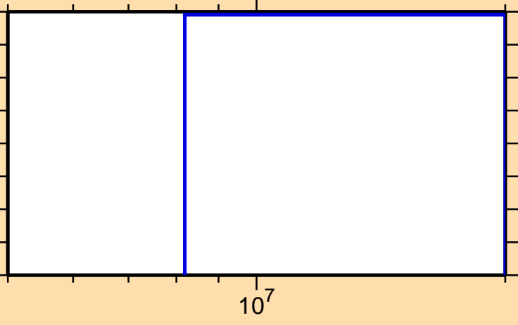
\sigma vs. E for ^{96}\text{Rh}(n,\text{pd})
