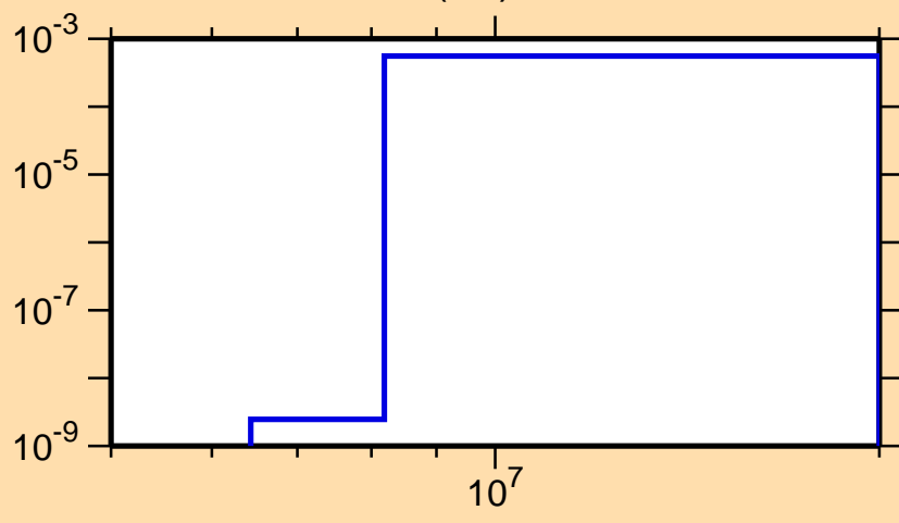
\sigma vs. E for ^{96}\text{Rh}(n,t)
