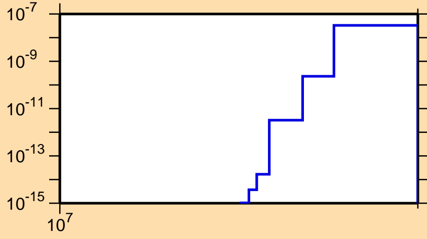
\sigma vs. E for ^{96}\text{Rh} (mt 34)
