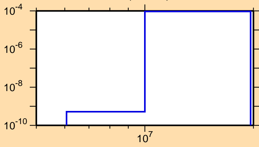
\sigma vs. E for ^{96}\text{Rh}(n,\text{He3})
