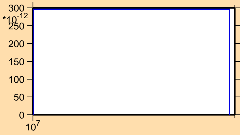
\sigma vs. E for ^{96}\text{Rh}(\text{mt } 34)
