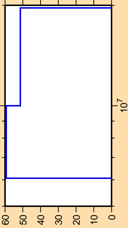
\Delta\sigma/\sigma vs. E for ^{96}\text{Rh}(n,2n)
