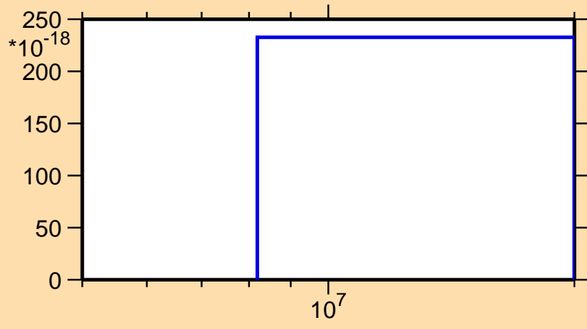
\sigma vs. E for ^{96}\text{Rh}(n,nt)
