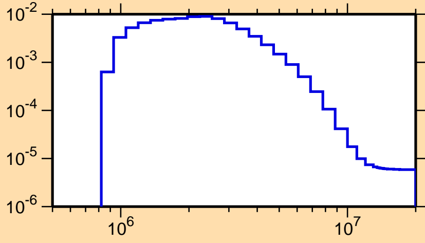
\sigma vs. E for ^{97}\text{Rh}(n,n_4)
