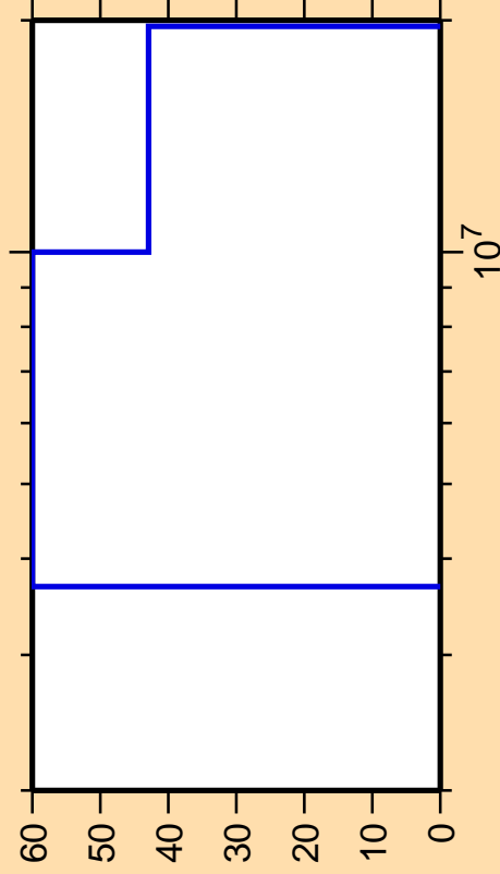
\Delta\sigma/\sigma vs. E for ^{97}\text{Rh}(n,n\alpha)
