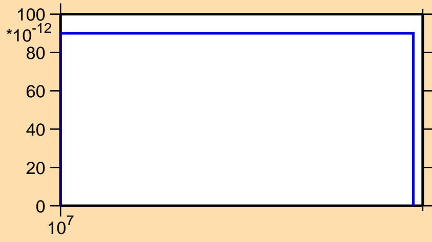
\sigma vs. E for ^{97}\text{Rh}(n,\text{pt})
