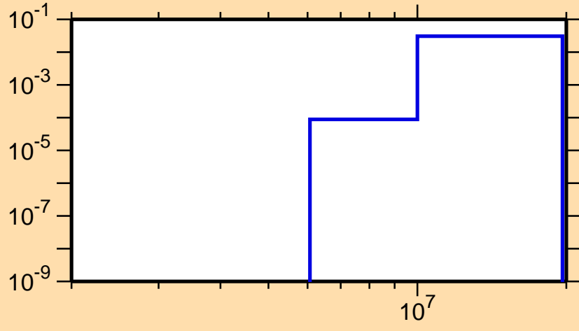
\sigma vs. E for ^{97}\text{Rh}(n,n\alpha)
