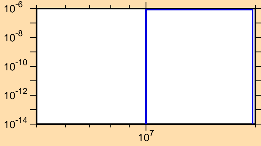
\sigma vs. E for ^{97}\text{Rh} (mt 45)
