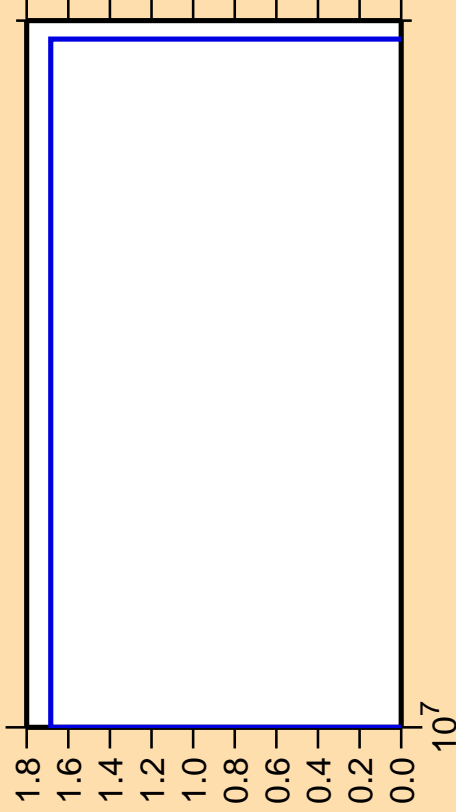
\Delta\sigma/\sigma vs. E for ^{97}\text{Rh} (mt 34)
