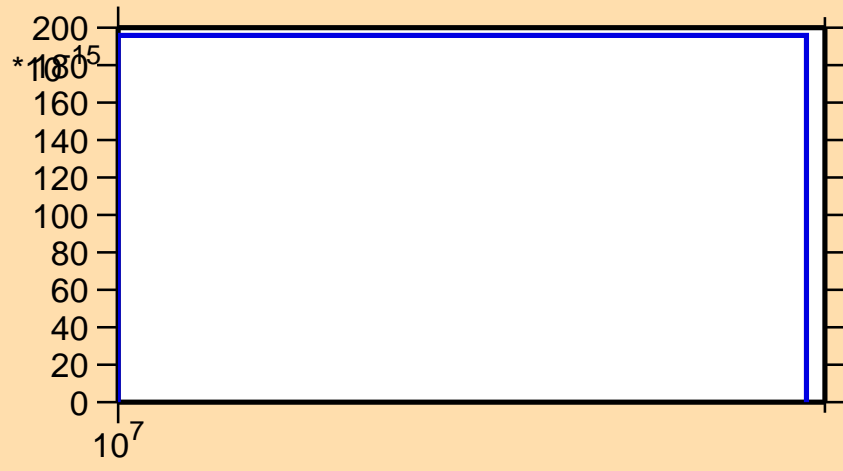
\sigma vs. E for ^{97}\text{Rh} (mt 34)
