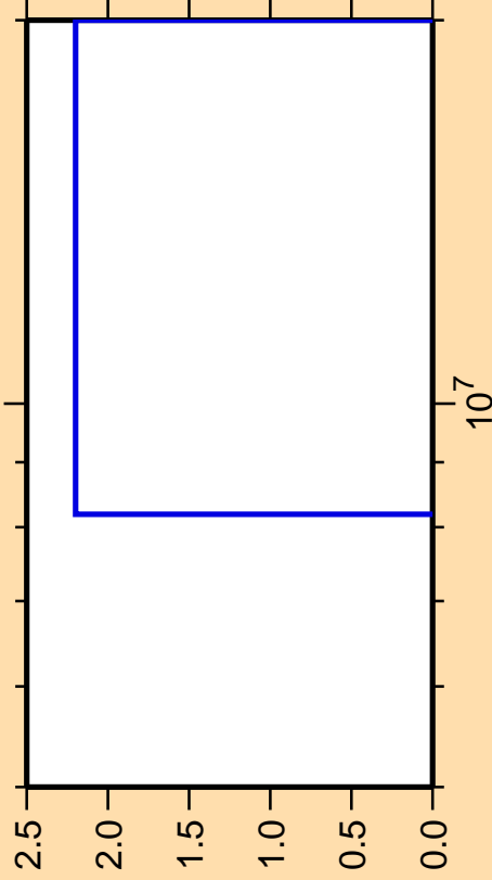
\Delta\sigma/\sigma vs. E for ^{97}\text{Rh}(\text{mt } 34)
