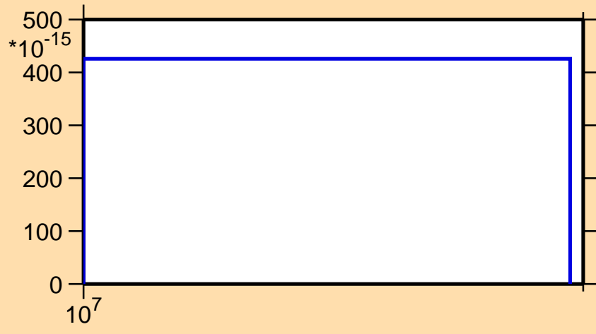
\sigma vs. E for ^{97}\text{Rh} (mt 34)
